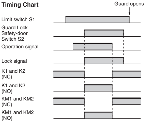
Timing Chart
